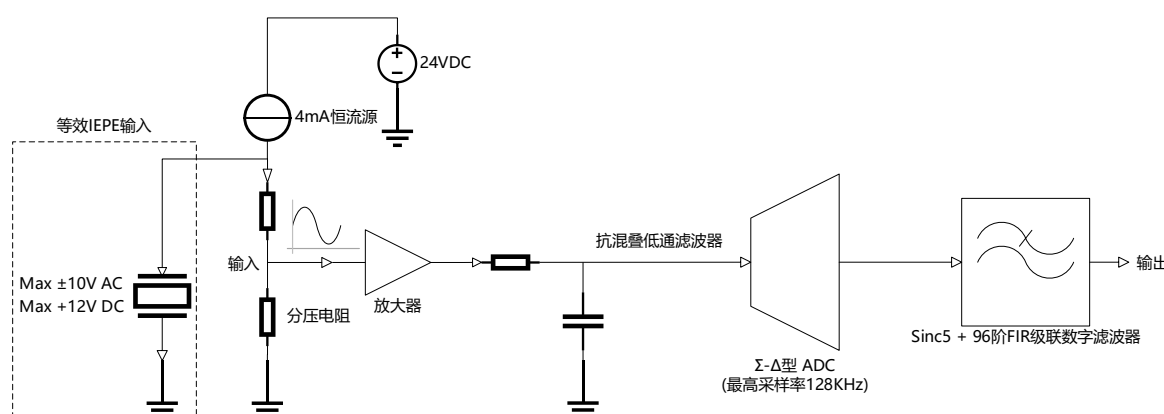
Figure 9-1 IEPE Signal Chain
