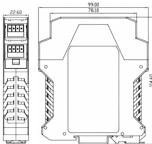
Figure 6-1 Mechanical Dimensions (unit: mm)
