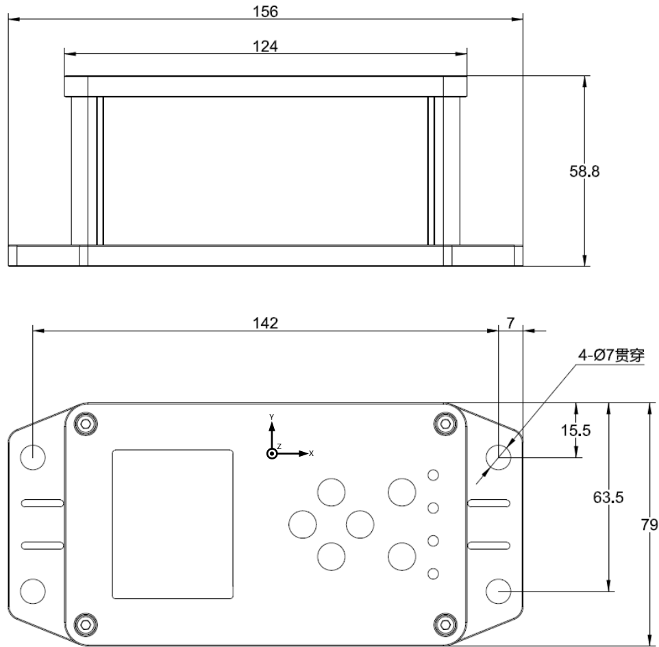
Figure 6-1 Mechanical Dimensions (unit: mm)
